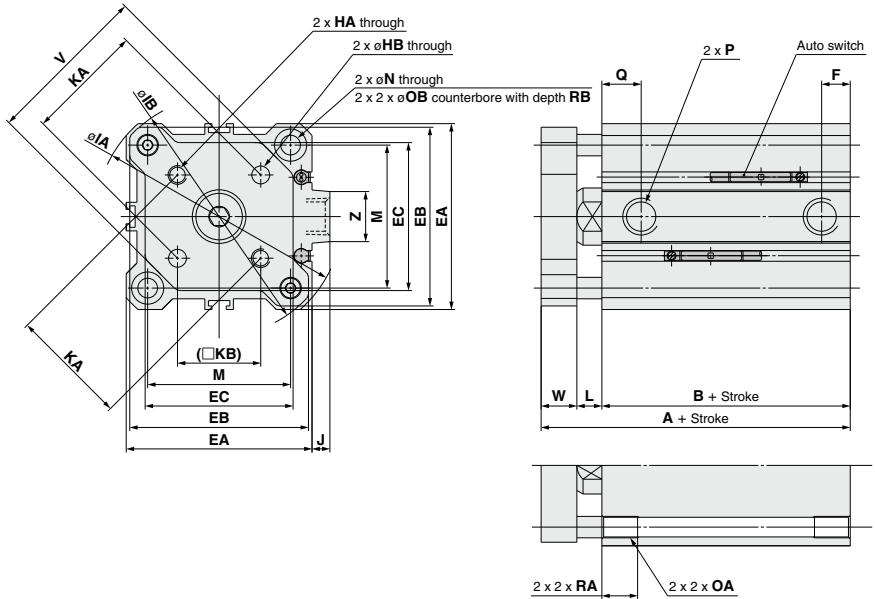
Both ends tapped (CQMA)
